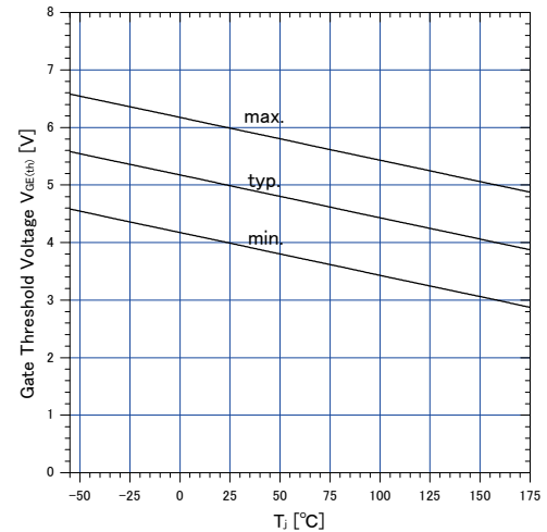
Graph.6 Gate Threshold Voltage vs. T_j I_c = 75mA, V_{GE} = 20V
